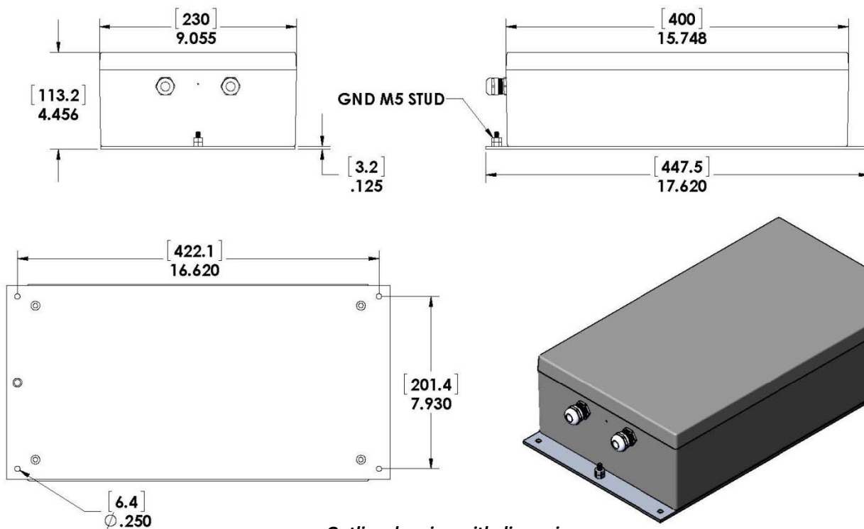
Outline drawing with dimensions
