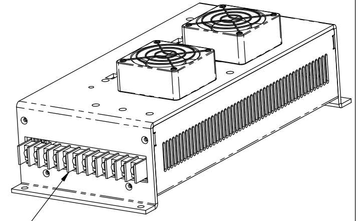
12 Pole barrier type of terminal with M3.5 screws
